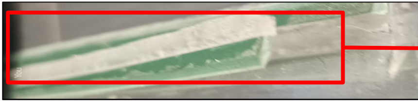
OLD CREASING MATRIX
